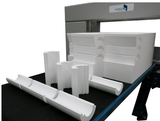
Typical Pipe Shells profiled and cut to length in one operation
